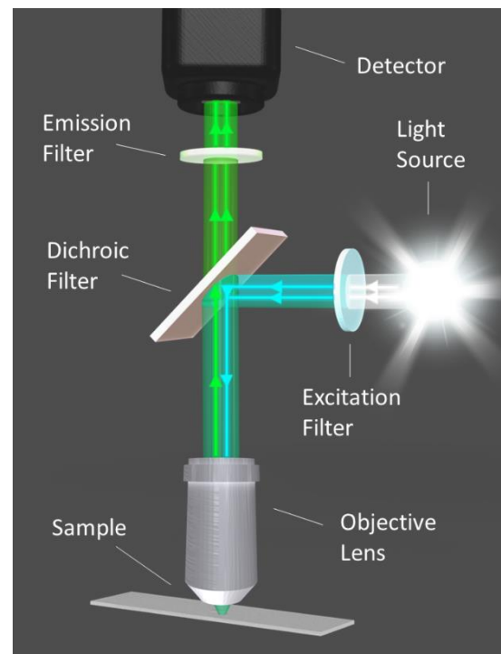
Work Principle of the Fluorescence Microscope
